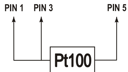
Input wiring schematic for Pt100 sensor with 3 wires.
